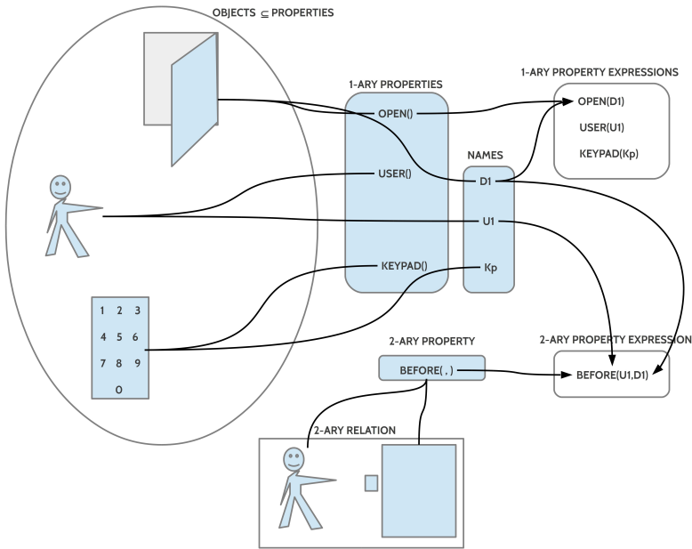
Figure 4.4: Example of a picture-to-math mapping for properties and objects
